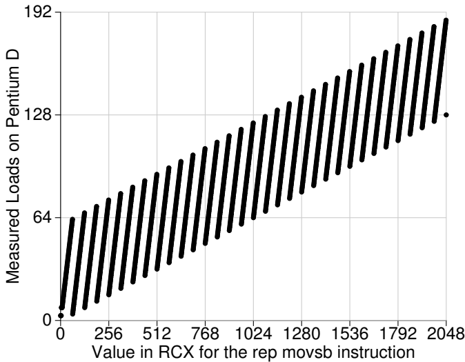
Fig. 1. On Pentium D, the retired loads event shows unusual behavior with rep movsb string instructions. The observed count is related to 64-byte chunks being moved with individual moves for the remainder: (\text{floor}(\text{reps}/64) * 4) + (\text{reps}\%64) .
