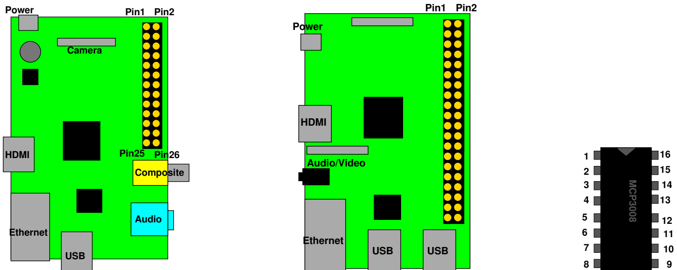
Figure 1: Location of header on Raspberry Pi Model B and B+/2/3, Pinout of MCP3008
