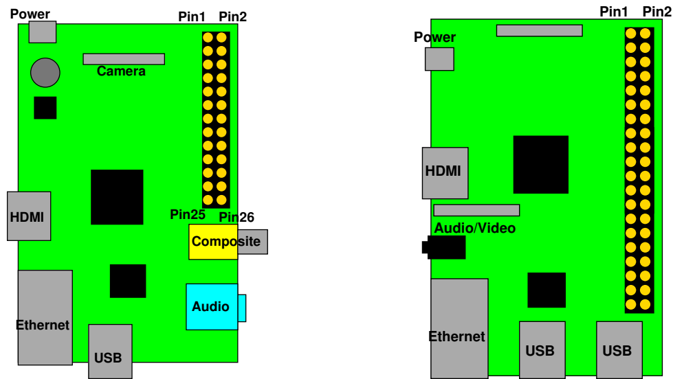
Figure 1: Location of header on Raspberry Pi Model B and B+
