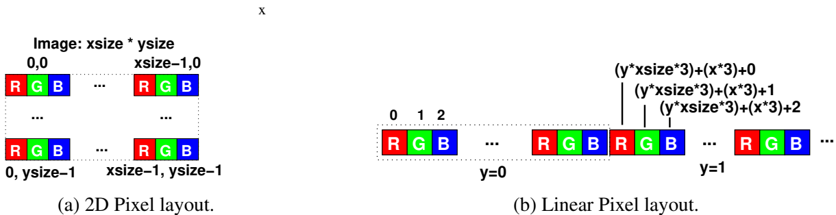
Figure 1: Image data memory layout
