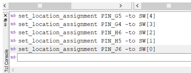
Figure 7: Tcl Console After Running Pin Assignments
